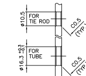
DETAIL "BAFFLE HOLE"
